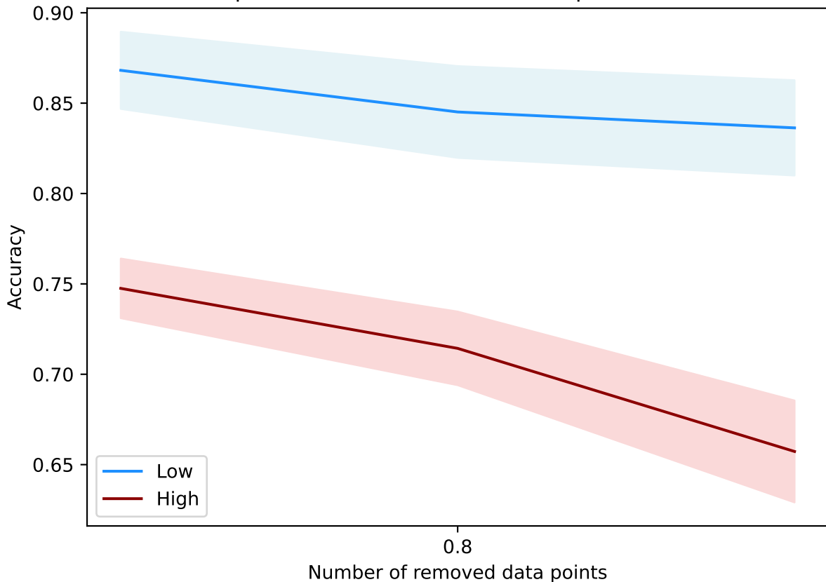
DataAttrOpt(10000, 0.2, 15, best, +b, alpha=best) - nomao
